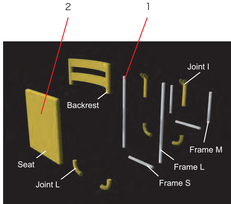
Parts Structure
